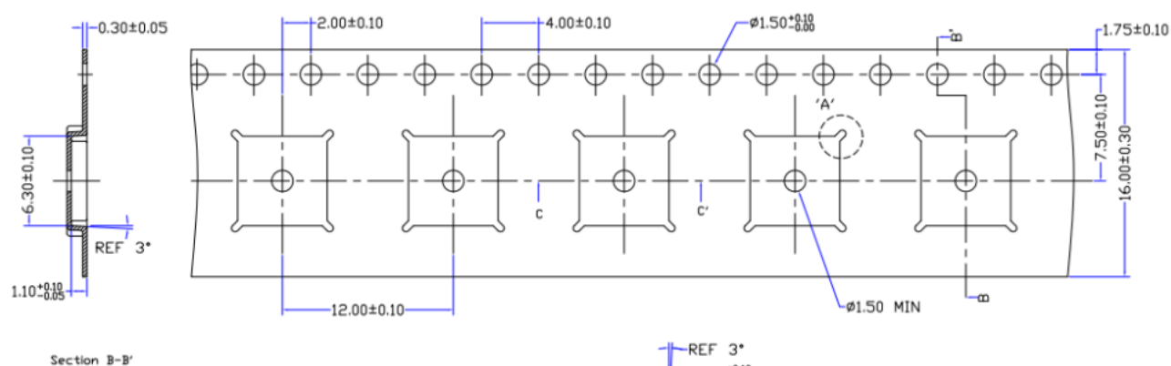
Section B-B'
