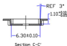
Section C-C'
